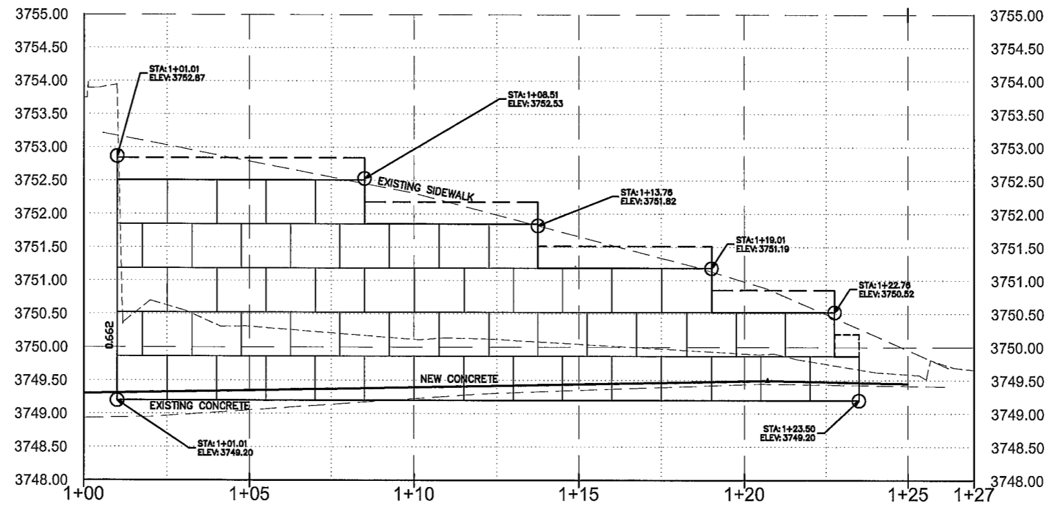
PROFILE Scale 1" = 4' Horiz. Scale 1" = 2' Vert.
